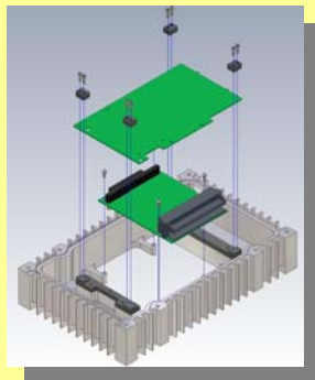
PCI to PC/104 Enclosure Systems
