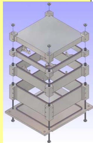
PC/104 and PC/104-Plus Enclosure Systems
