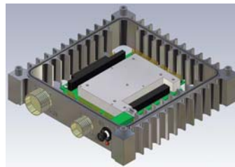
SBC mounted in dual-height ring
